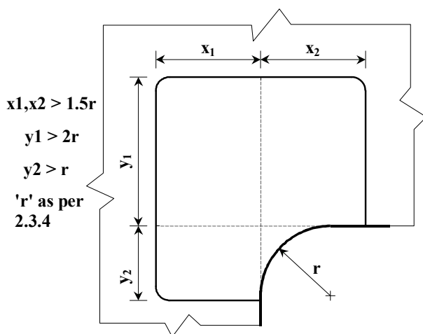
Fig.3.4.4 : Extent of insert plate
