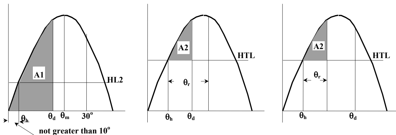
Fig.1 : Intact Stability
