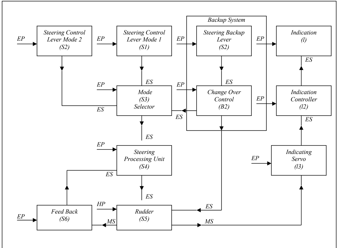
Fig.1 : Example of a system block diagram
