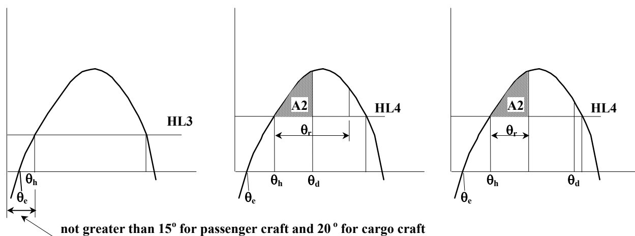
Fig. 2 : Damage Stability
