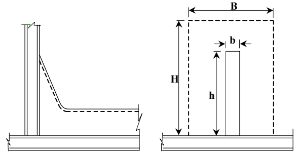
Fig. 9.2.4: Effective bond area
